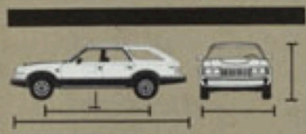
EAGLE WAGON DIMENSIONS (inches unless otherwise specified)
